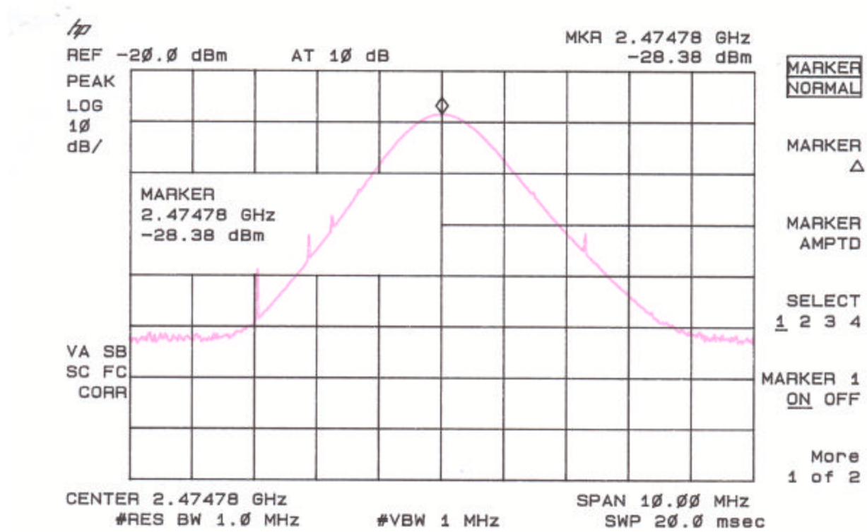
Figure 4c - 1 Peak Radiated Spurious Emission 15.247(c) Fundamental High
