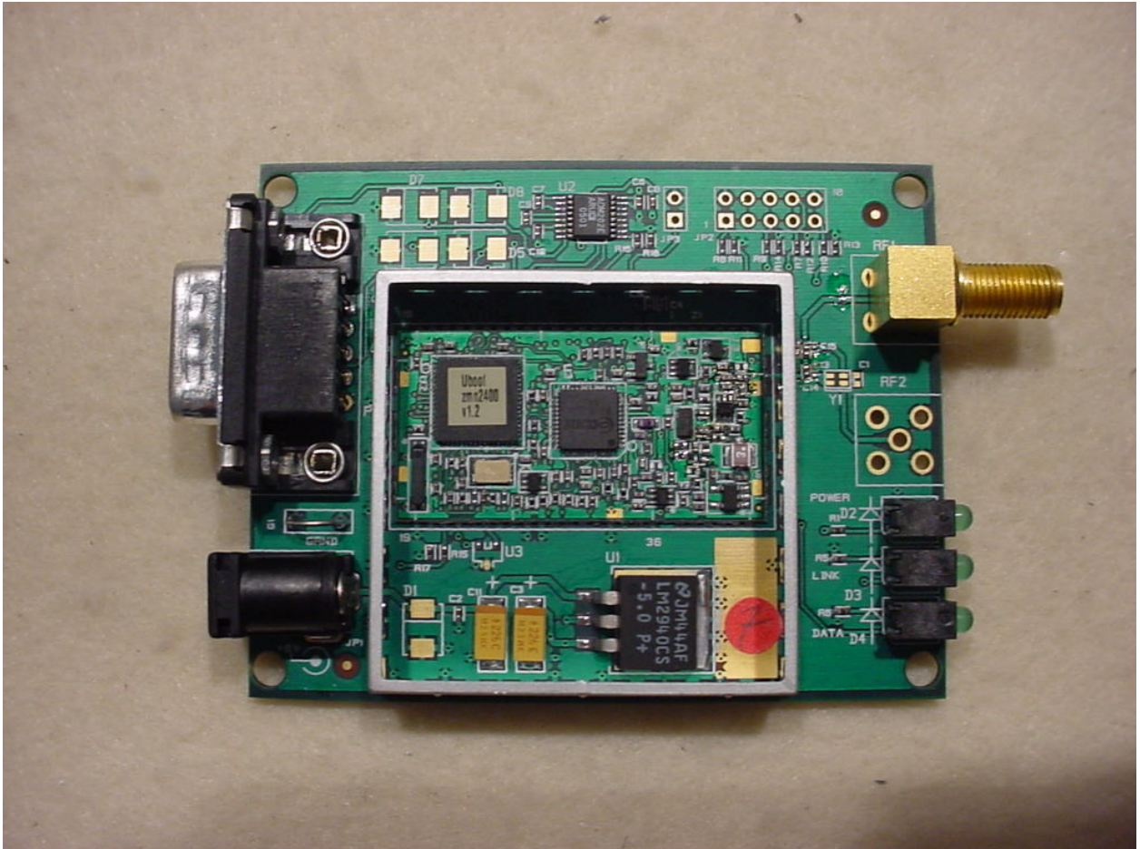
Figure 2: Internal – Top View without Shield
