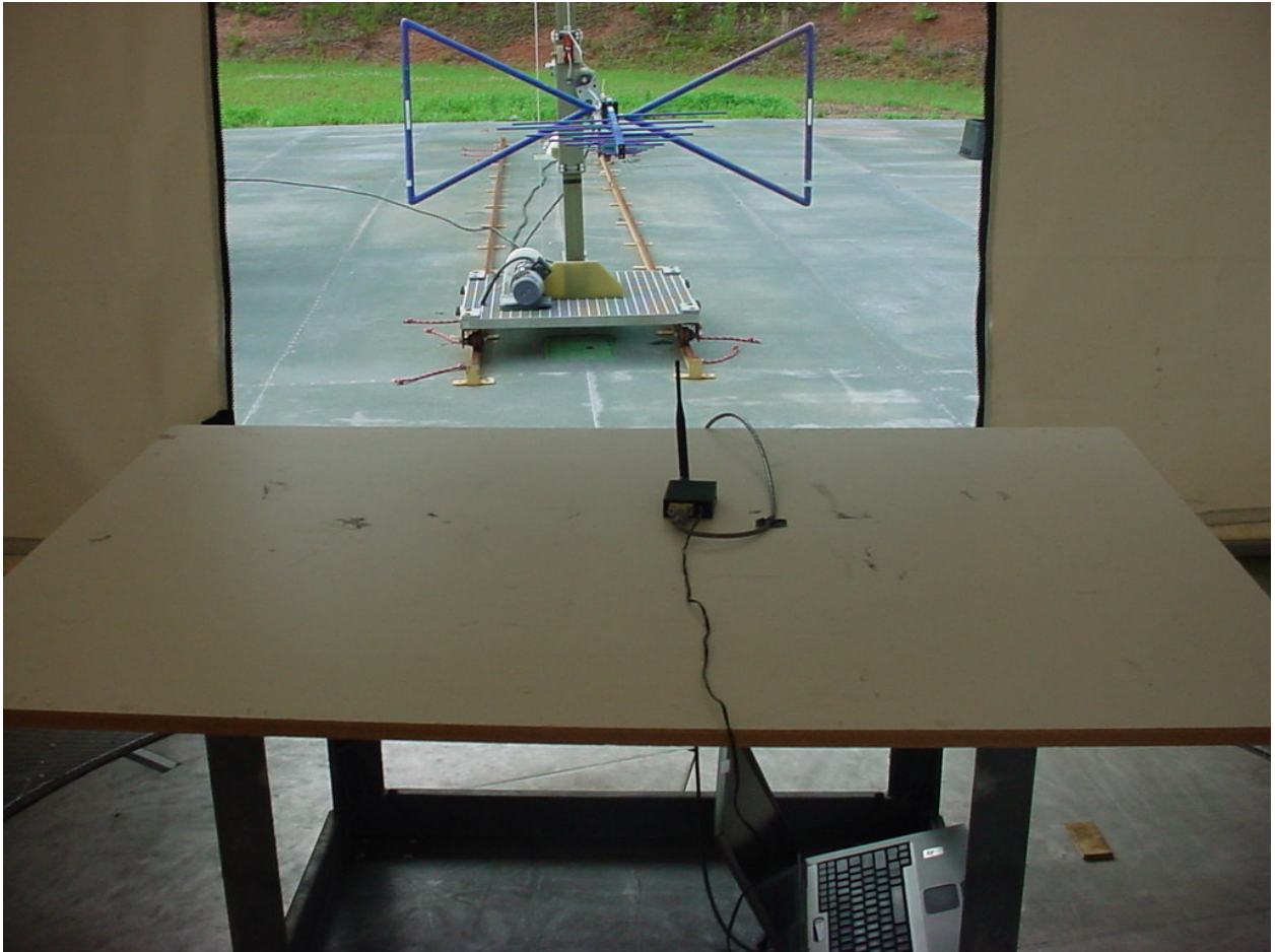
Figure 2: Unintentional Radiated Emissions – Rear View
