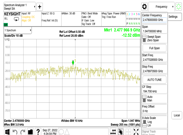
PSD_BLE 2M_HighCH38-2478MHz
