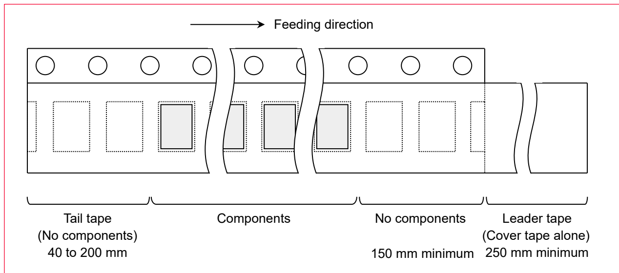
Figure 8: Leader and Tail Tape
