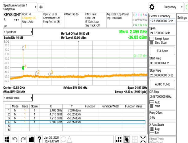
Spurious Emission_Zigbee_LowCH11-2405MHz
