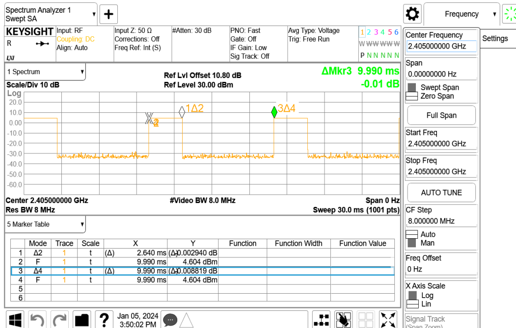
Zigbee_LowCH11-2405
