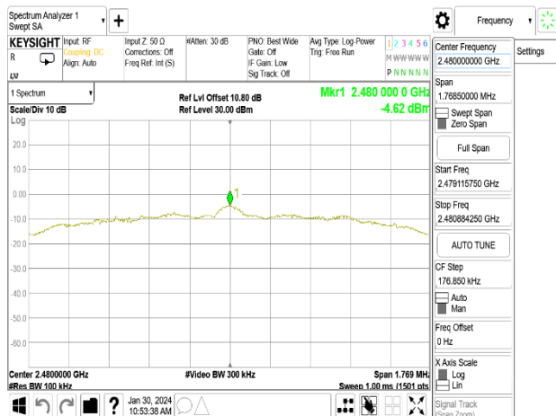
Reference Level_Zigbee_HighCH26-2480MHz
