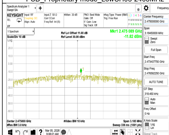
PSD_Proprietary mode_HighCH75-2475MHz
