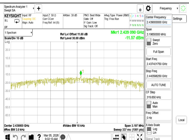
PSD_Proprietary mode_MidCH39-2439MHz
