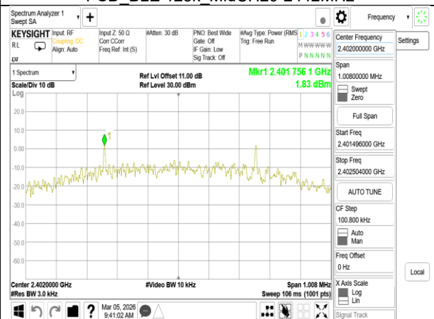
PSD_BLE 500k_LowCH00-2402MHz
