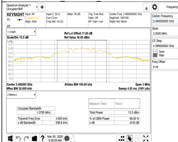
IC OBW_BLE 125k_HighCH39-2480MHz
