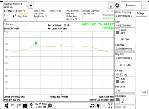
Reference Level_BLE 500k_LowCH00-2402MHz
