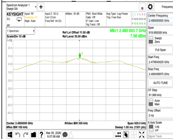
Reference Level_BLE 125k_HighCH39-2480MHz
