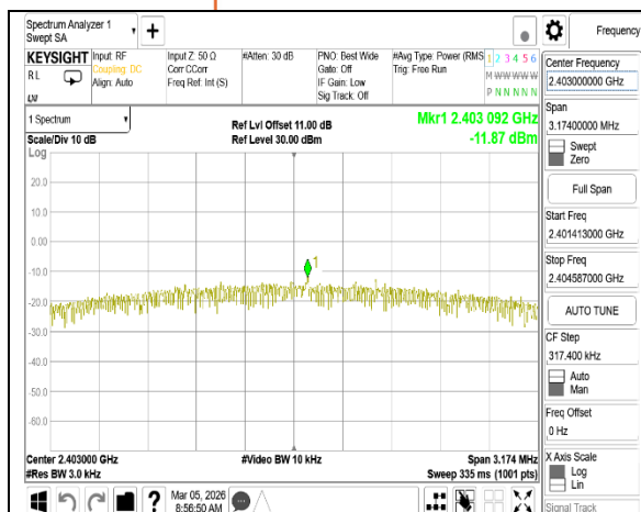
PSD_Proprietary mode_LowCH03-2403MHz
