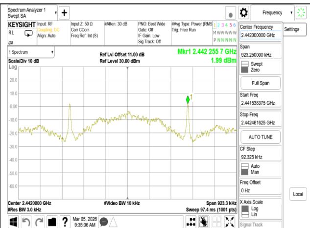
PSD_BLE 125k_MidCH20-2442MHz
