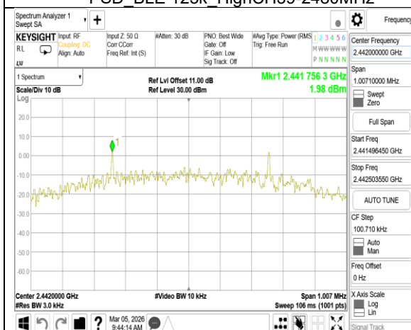
PSD_BLE 500k_MidCH20-2442MHz
