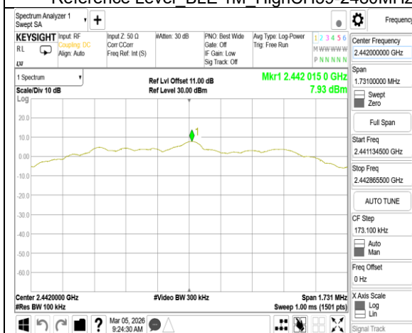
Reference Level_BLE 2M_MidCH20-2442MHz
