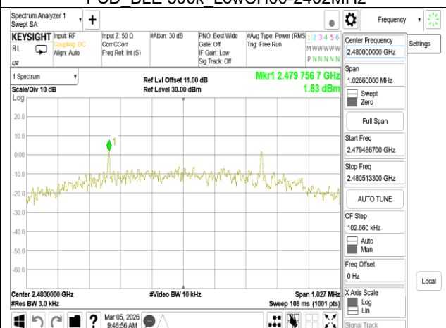
PSD_BLE 500k_HighCH39-2480MHz
