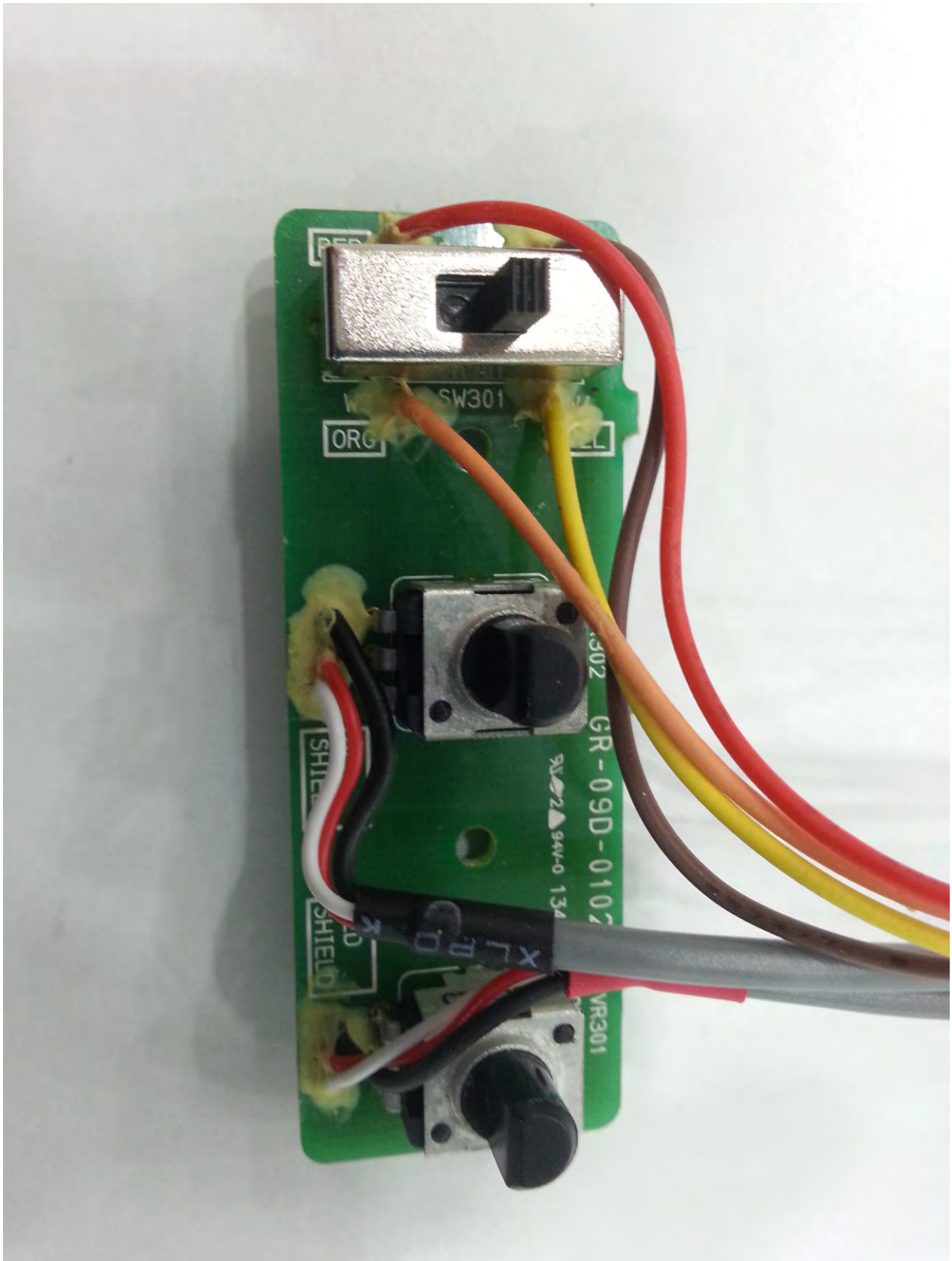
< Keypad Front >
