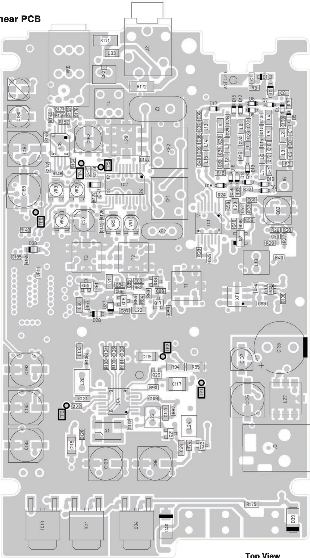
Top View
