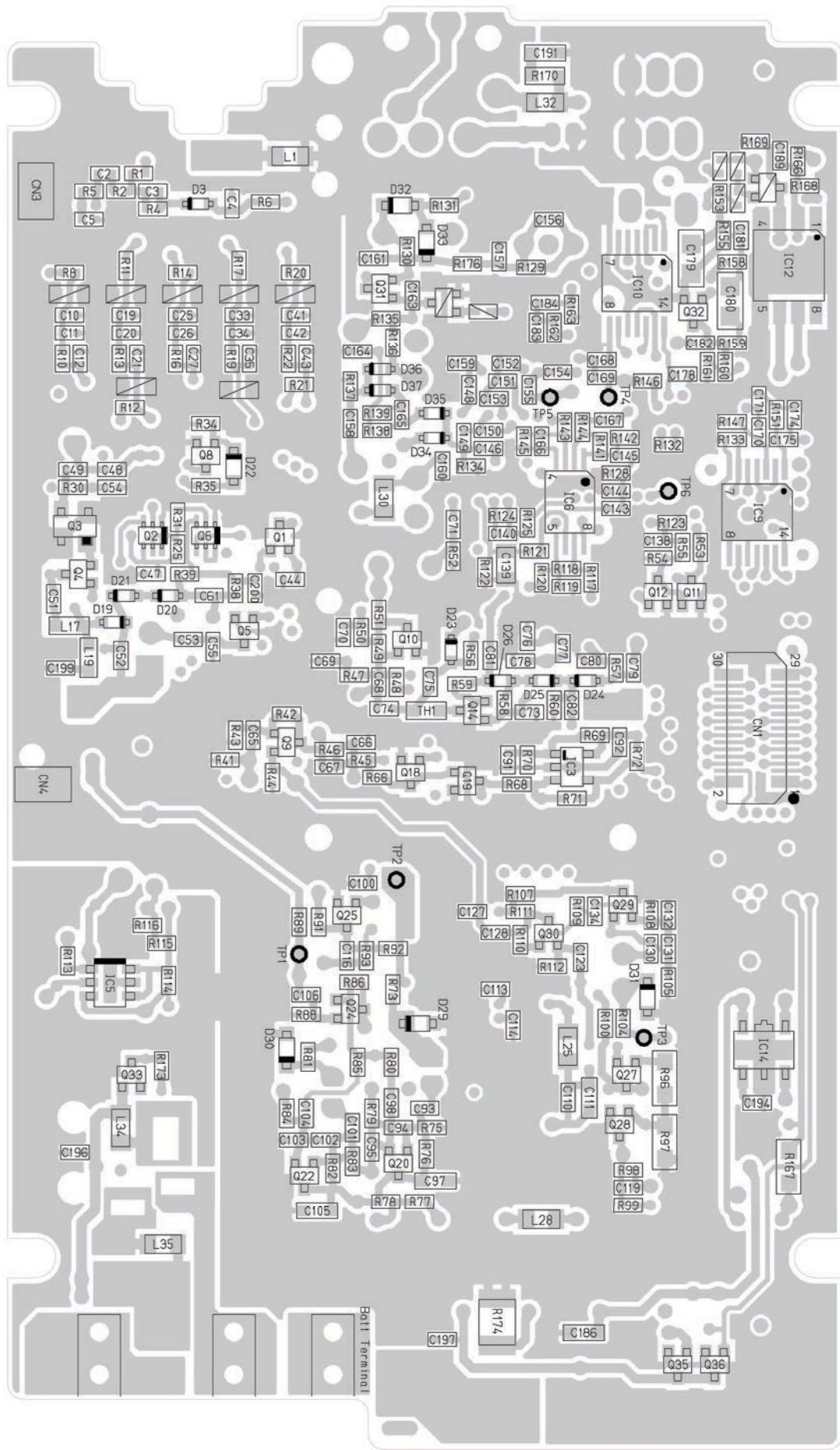
Bottom View
