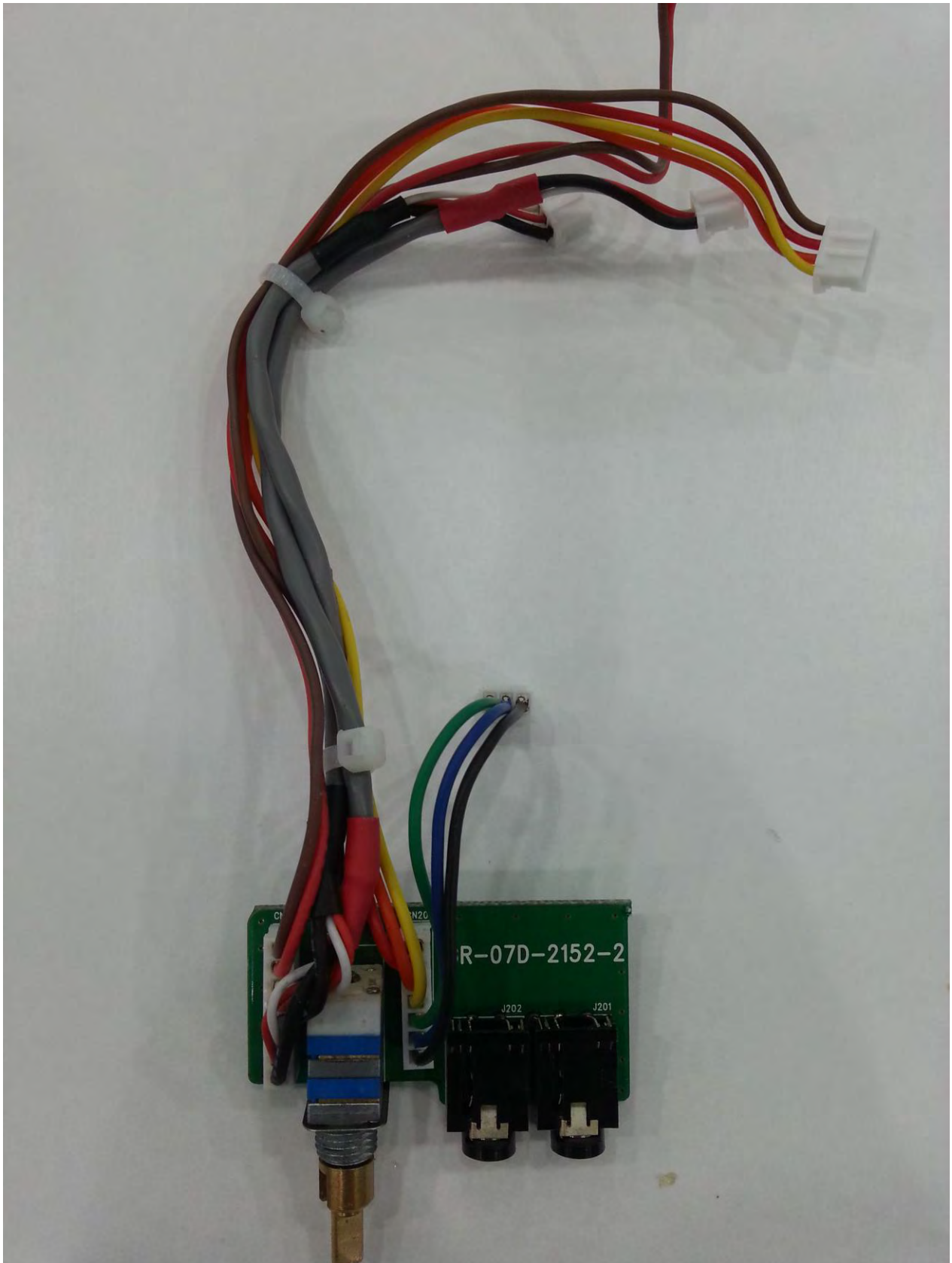
< Vol SQ Board Front >
