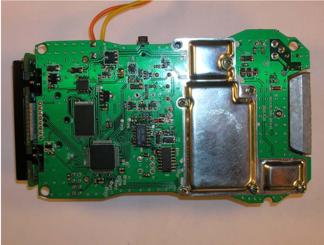
XTR-560 PCB bottom view
