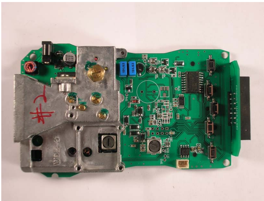
XTR-325 PCB top view
