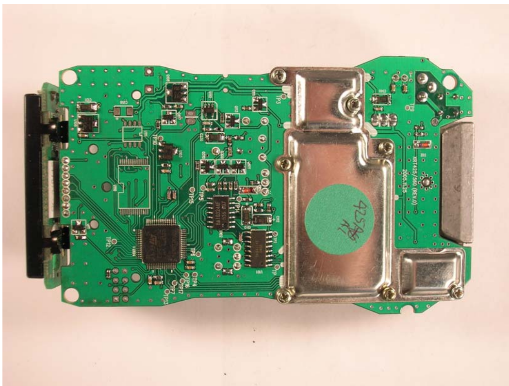
XTR-425 PCB bottom view
