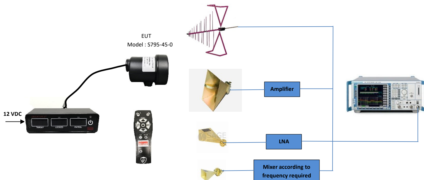
Figure 3.5-1: EUT Test Setup
