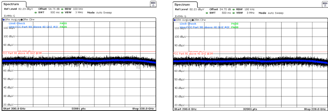
Figure 7.4-16: Radiated emissions plot – Field strength measured from 200 to 220 GHZ at 100 KHZ RBW, Rx antenna in horizontal and vertical polarization, respectively @3M.
