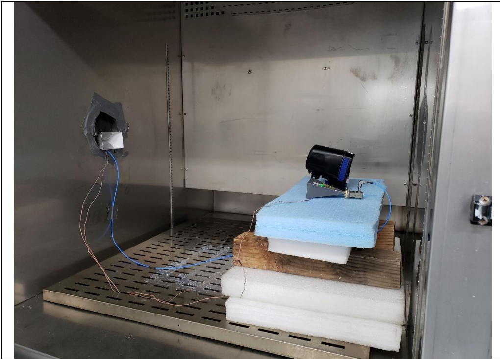
Frequency Stability #2
