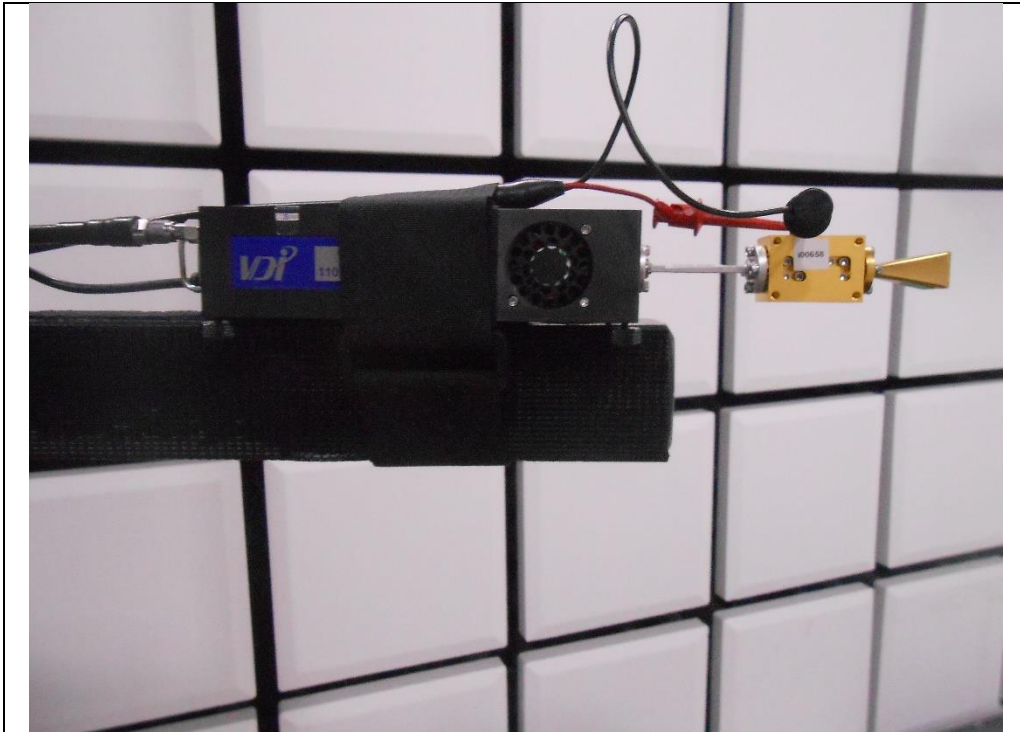
RF Radiated_ 110 - 170 GHz
