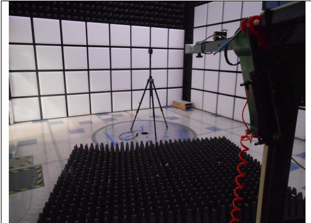
RF Radiated_ 40 – 50 GHz
