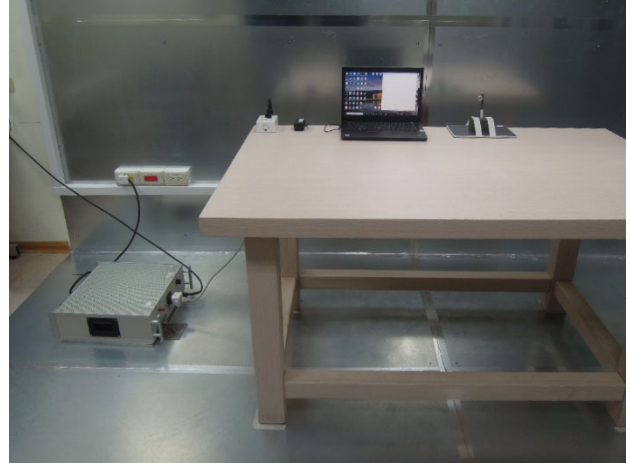
FCC_EMR_Conduction_Setup
