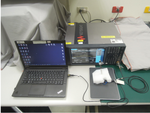
FCC_EMR_Radiated_Setup
