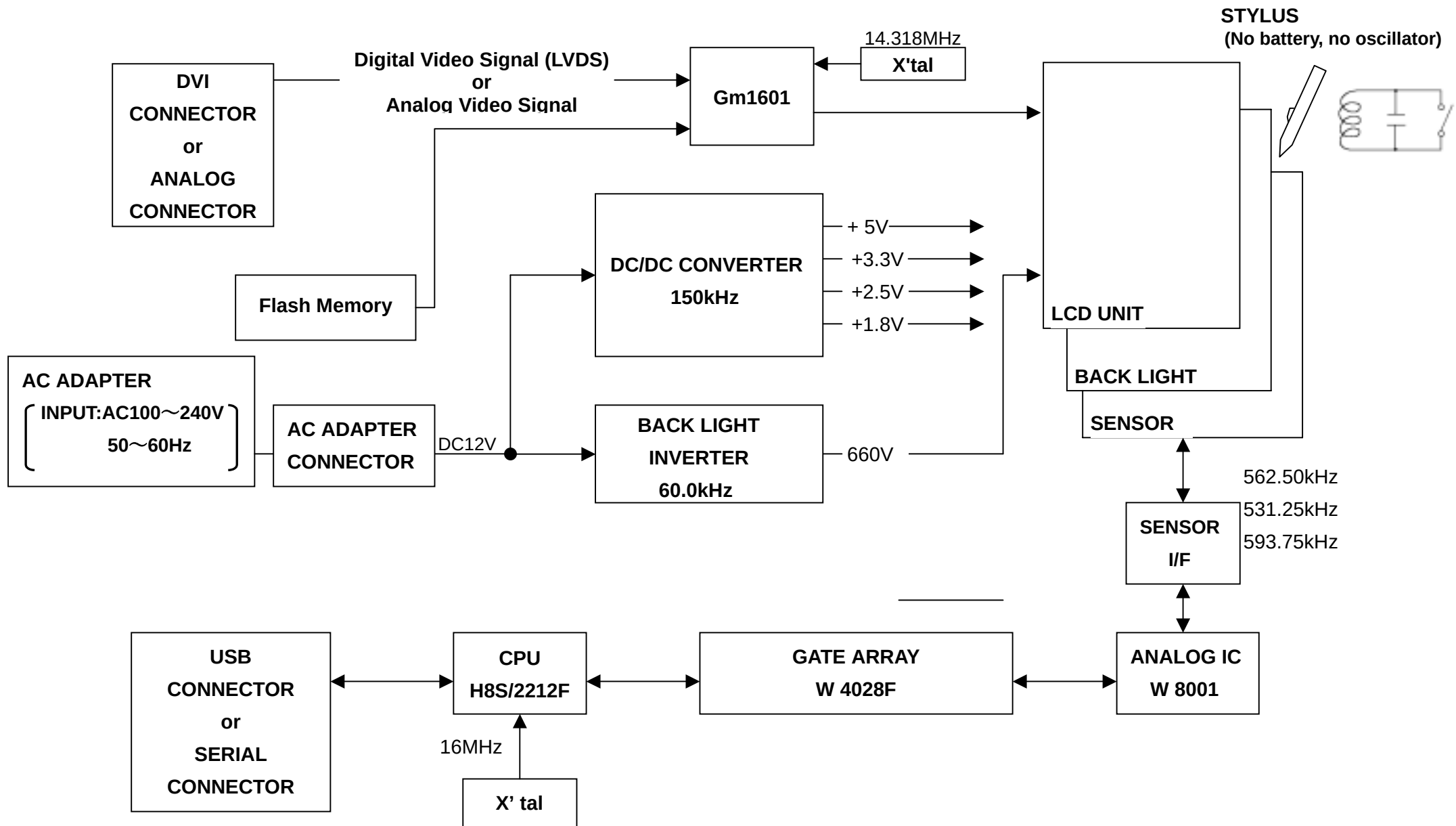
< DTU-710 Block Diagram >
