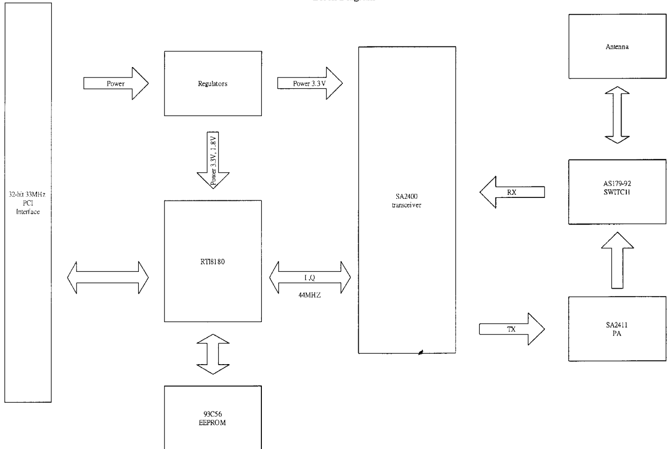
MUSTLINK01BC Block Diagram
