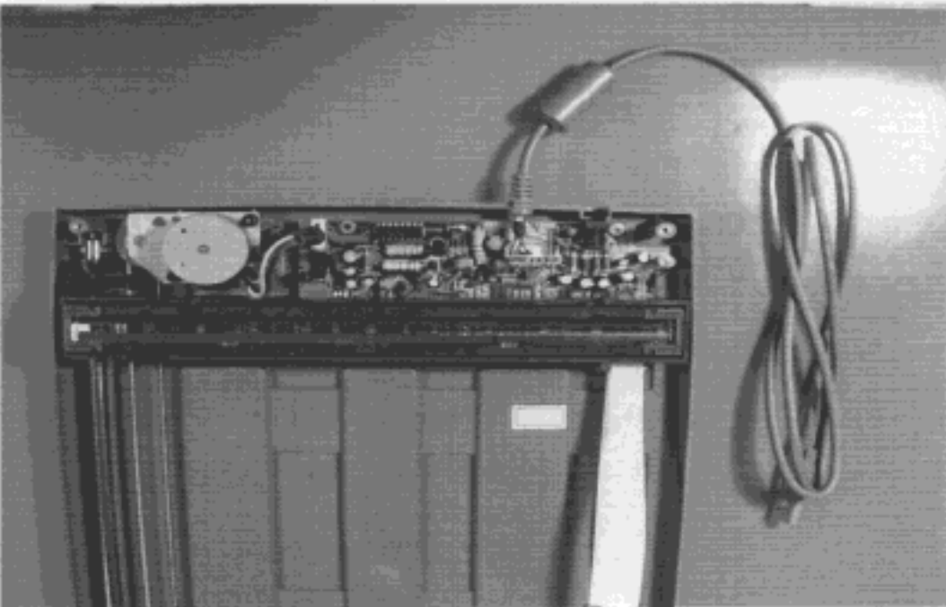
(5) INNER VIEW OF EUT
