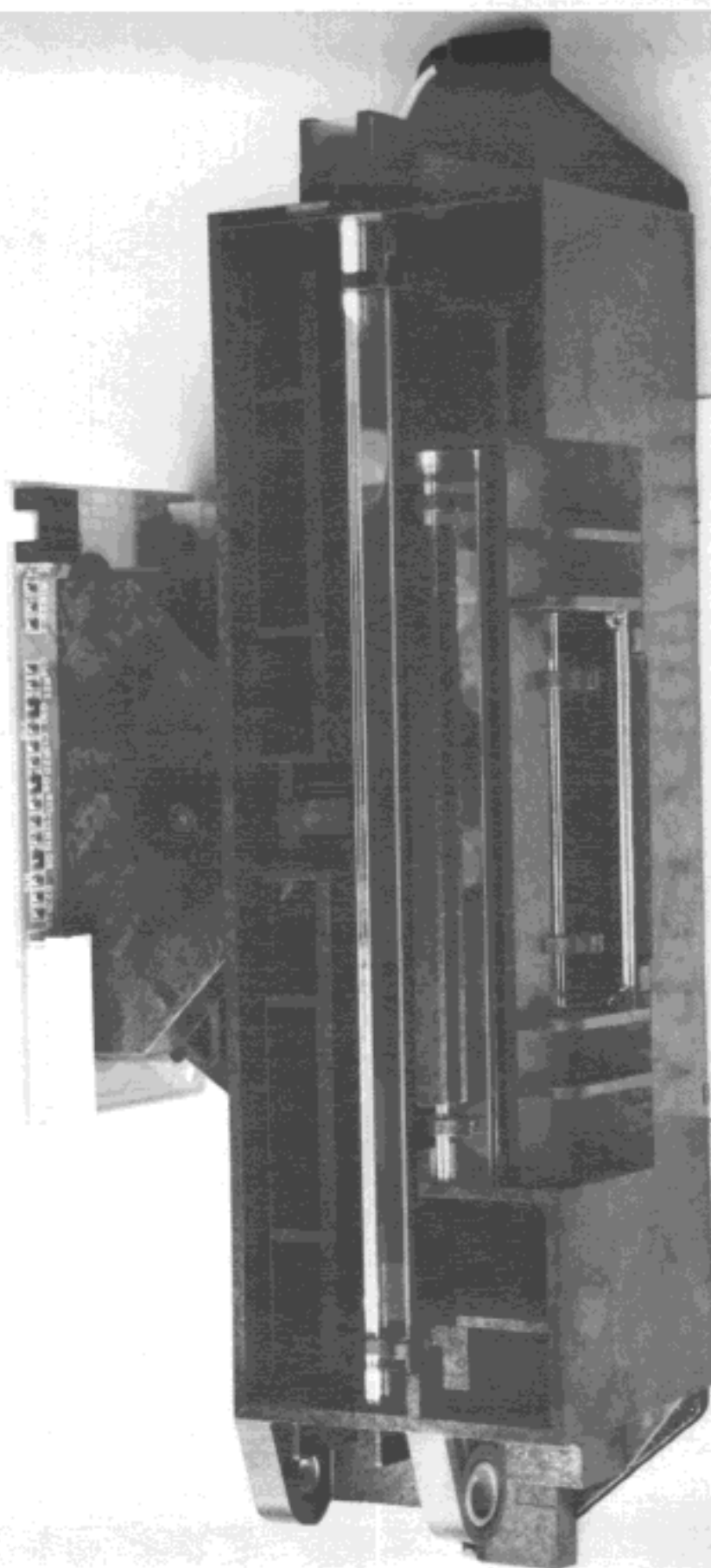
Figure 3 Scan Sensor Head w/CCD Board
