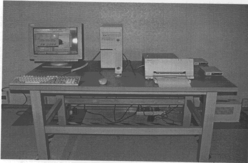
Mode 2 :Front View of Conducted Test ( Maximum Testing Configuration)
