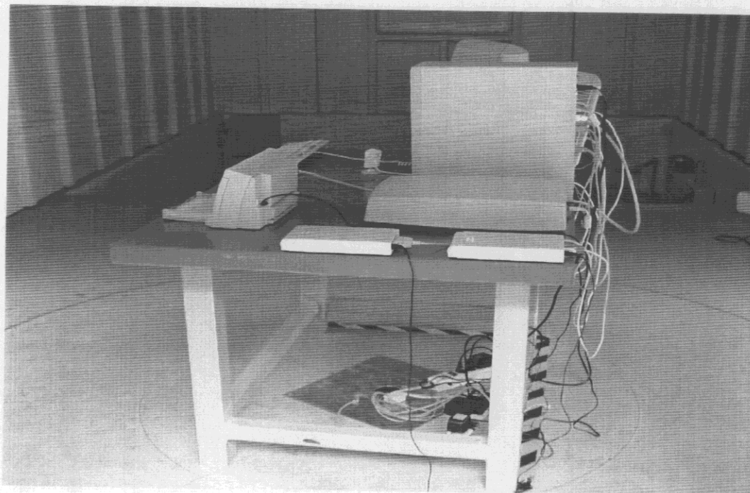
Mode 2 : Back View of Radiated Test (Maximum Testing Configuration)
