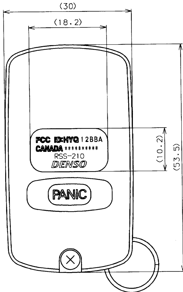
Fig. Marking location and layout of Transmitter
