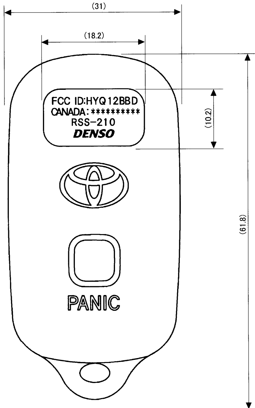
Fig. Marking location and layout of Transmitter
