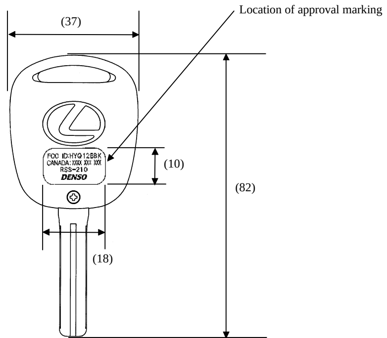
Fig. Marking location and layout of Transmitter
