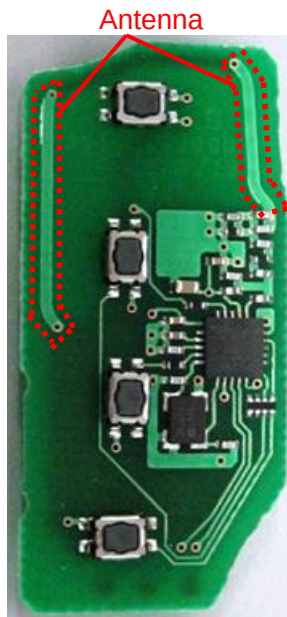
Component Side
