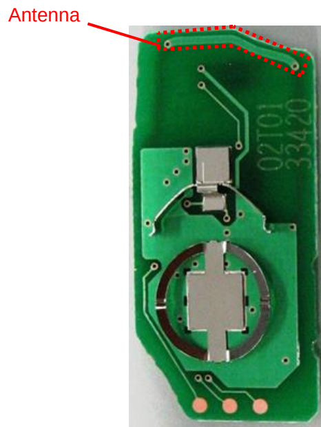
Solder Side
