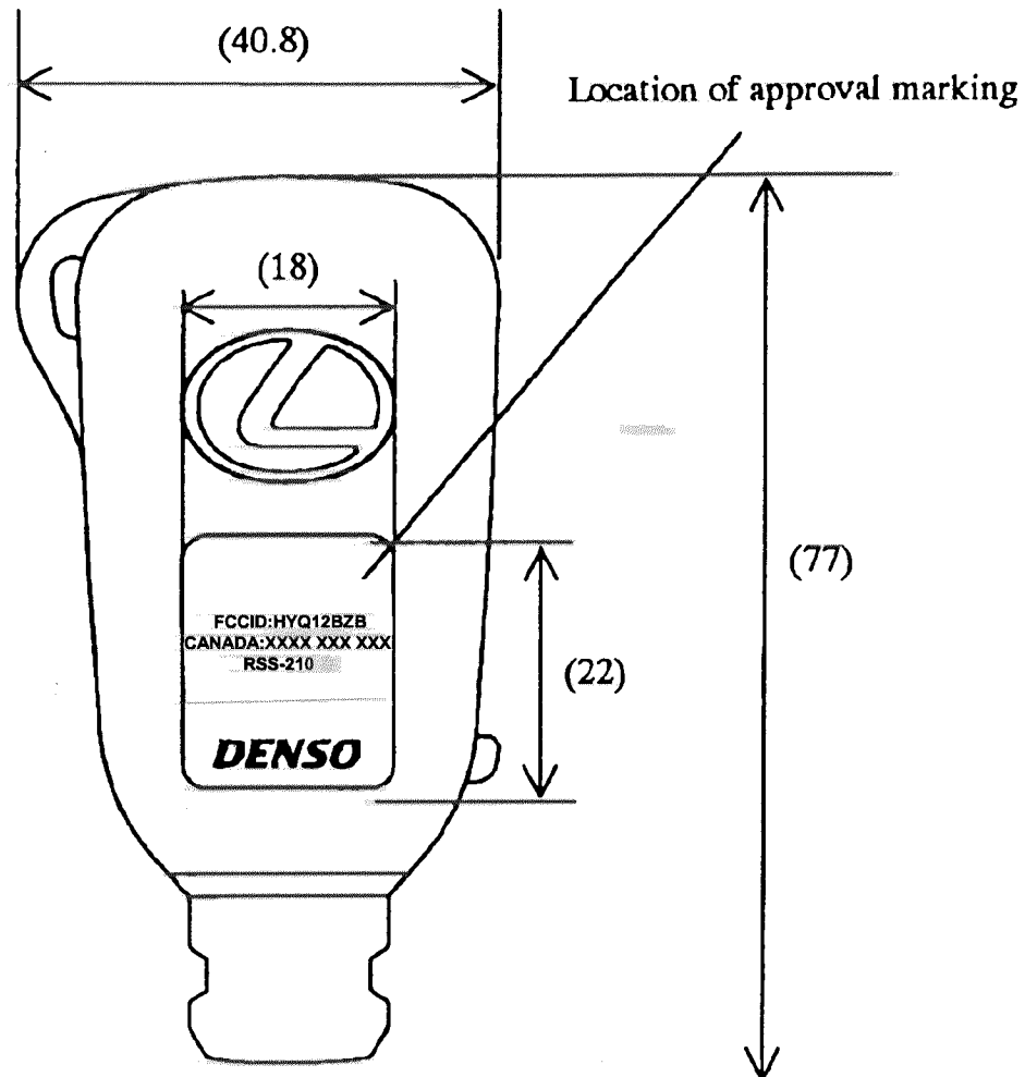
Fig. Marking Location and Layout of Transmitter
