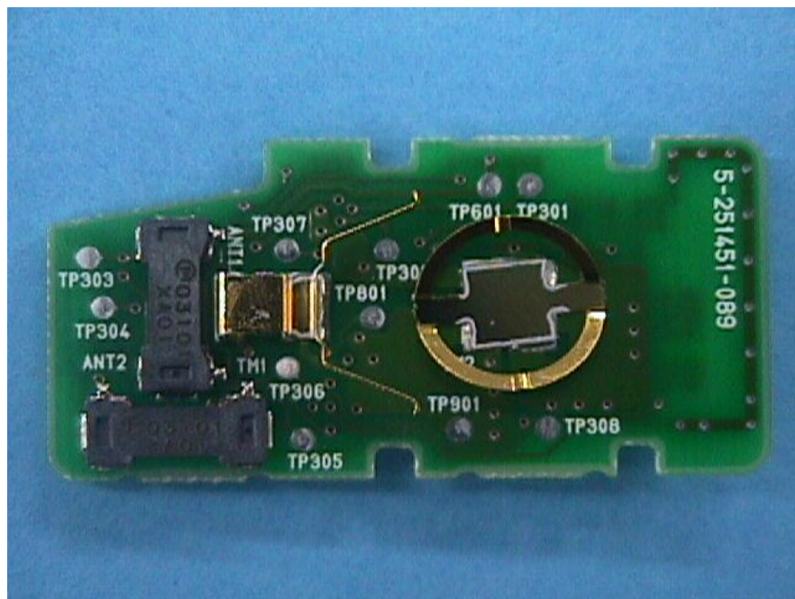
Circuit Board (rear)
