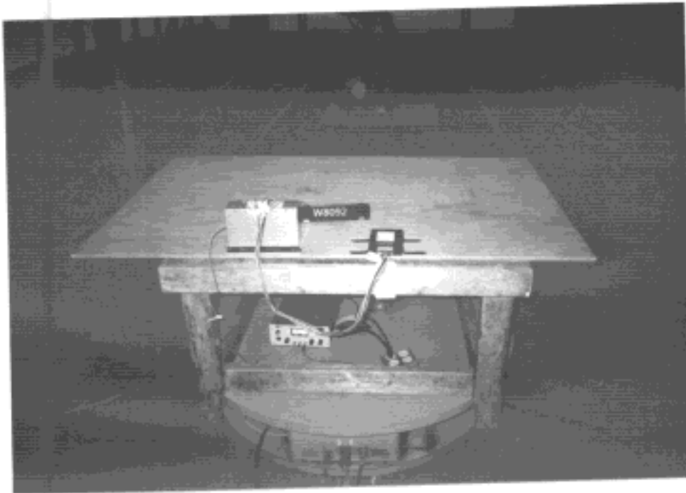
Test-setup photo(s): Radiated emission 30 MHz - 2000 MHz
