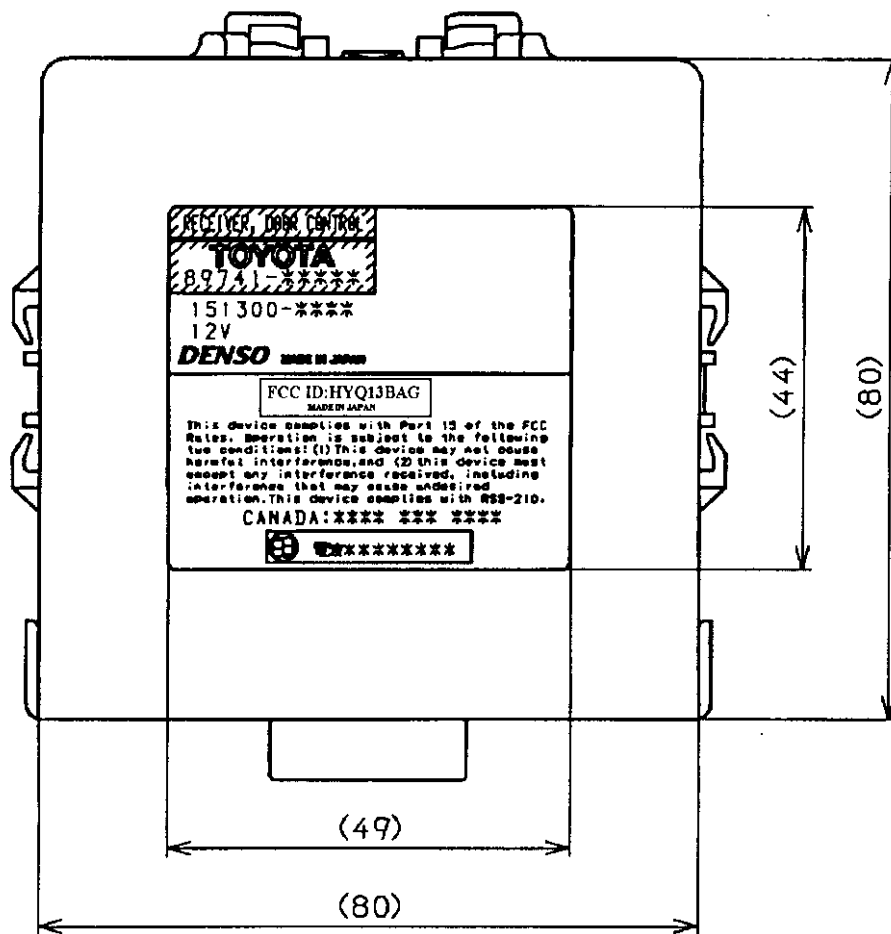
Fig. Marking location and layout of receiver
