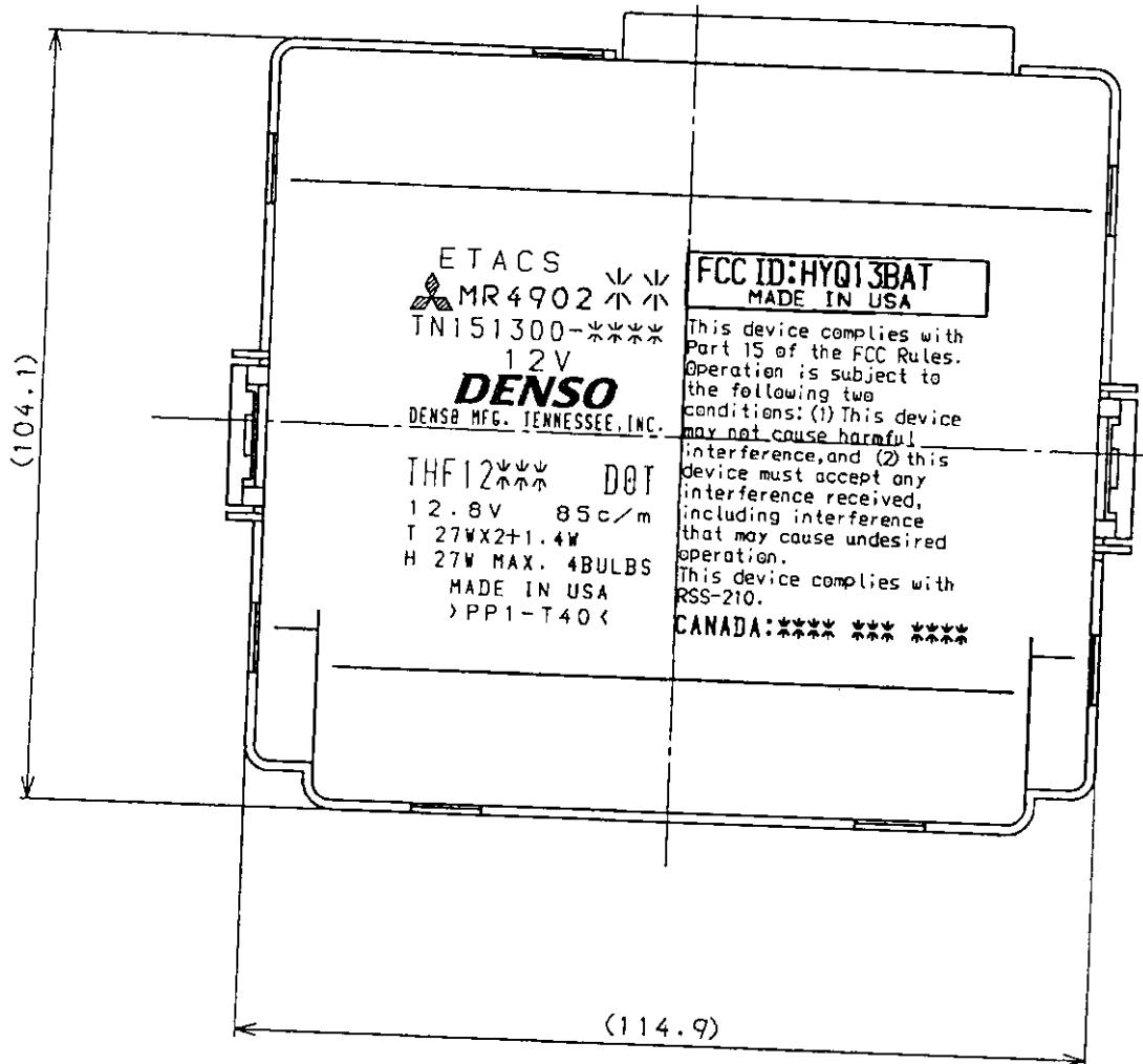
Fig. Marking location and layout of receiver
