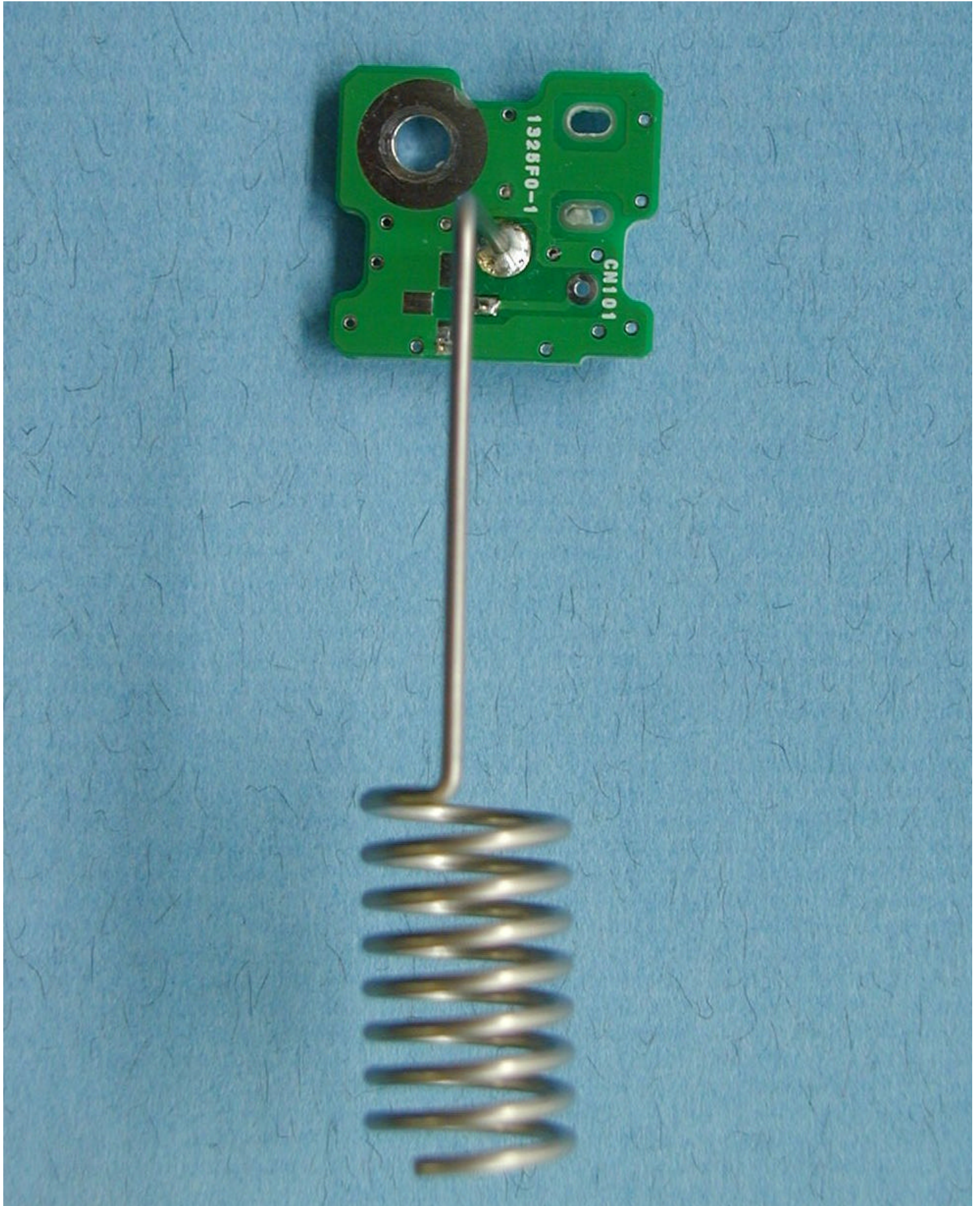
PCB Component side View of Antenna
