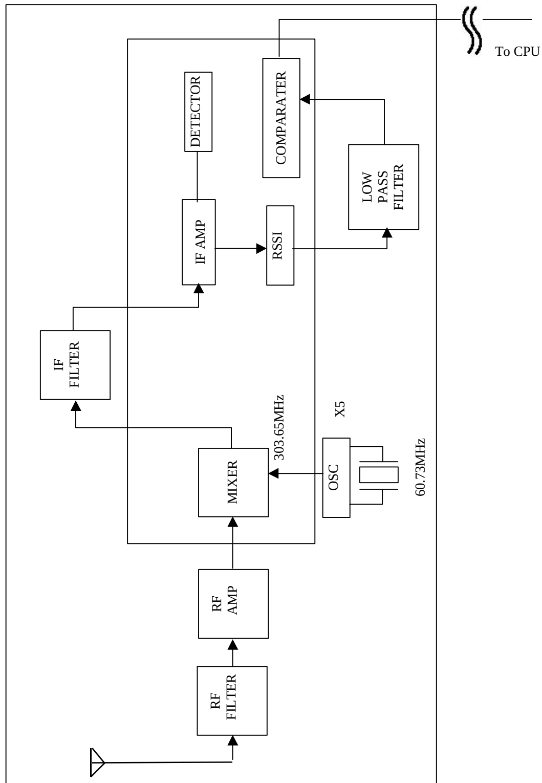
Fig. Block diagram of receiver
