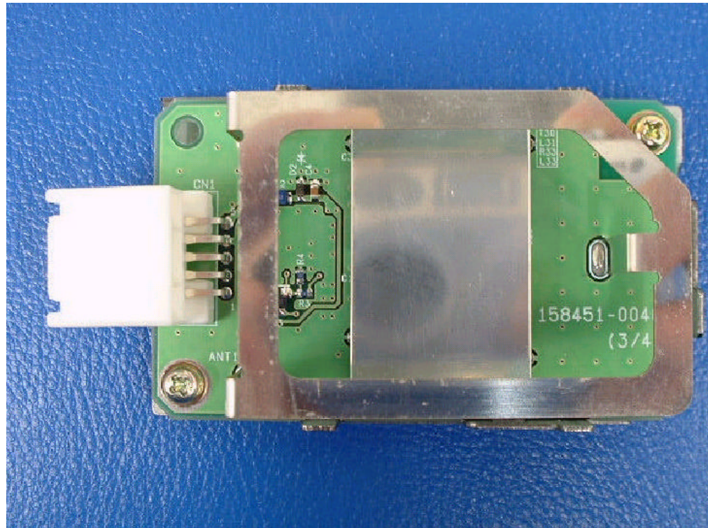
PCB Component side View of Receiver
