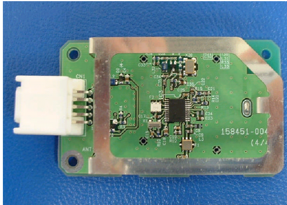
PCB Component side View of Receiver (without cover)
