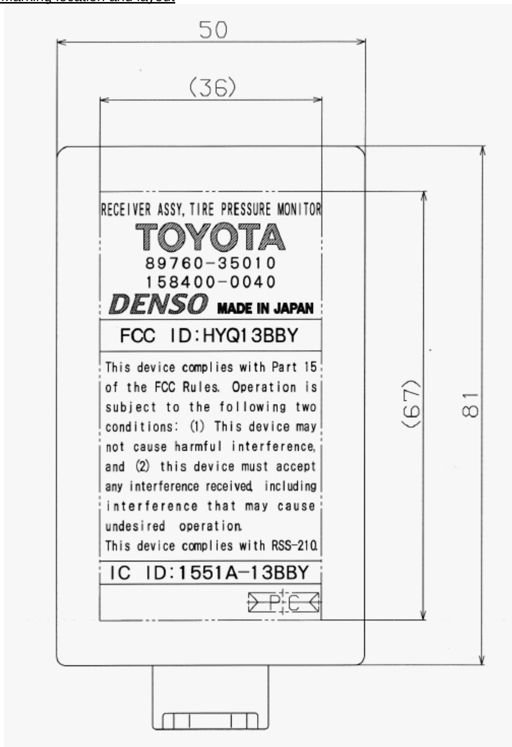
Fig7-1. Marking location and layout of receiver
