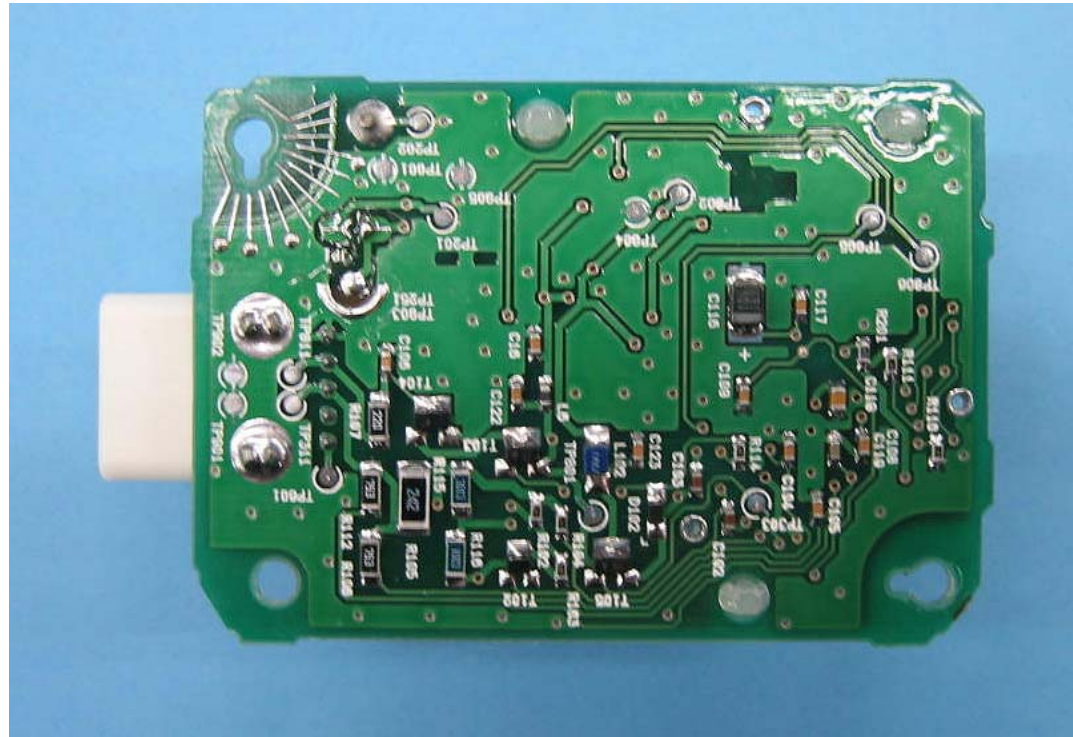
PCB Solder side View of Receiver
