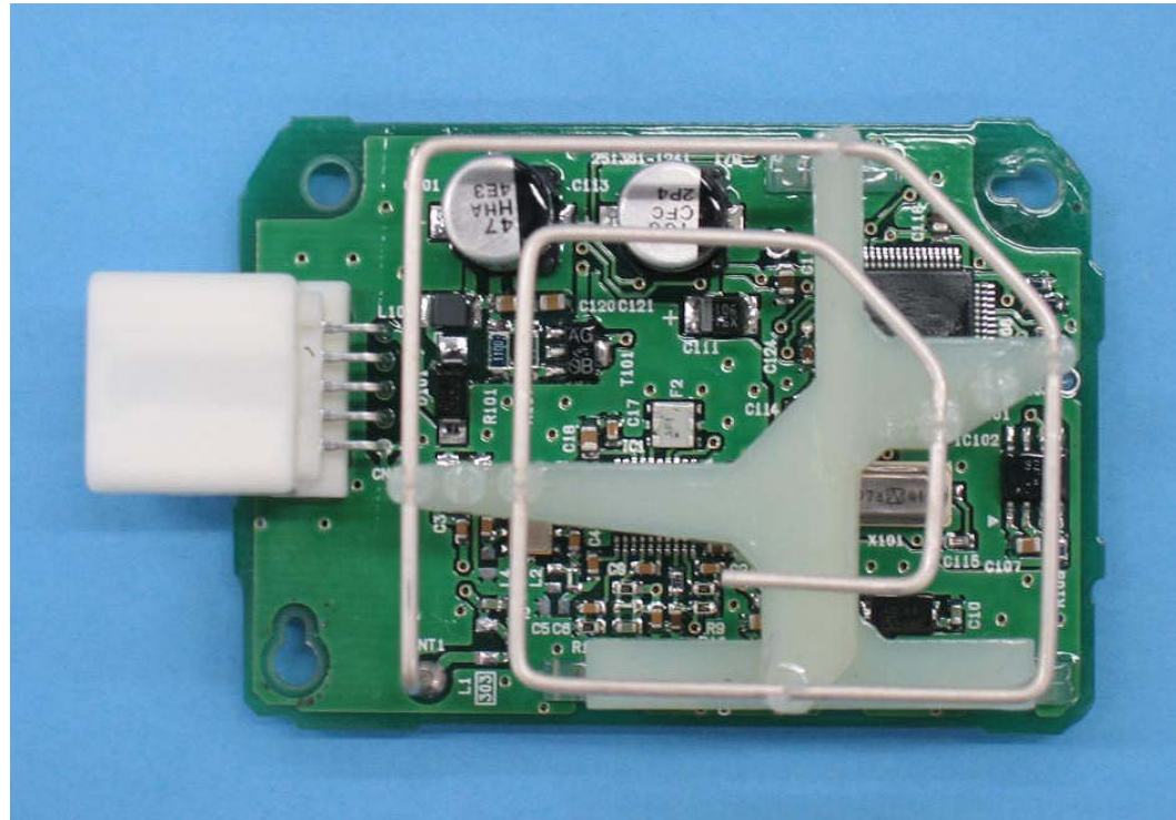
PCB Component side View of Receiver
