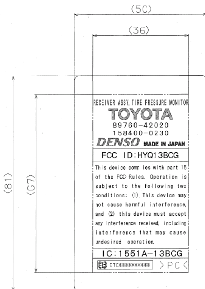
Fig7-1. Marking location and layout of receiver
