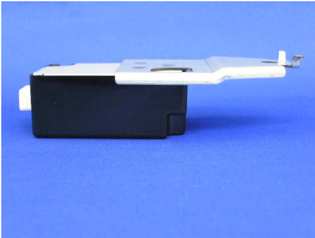
Side view 2
