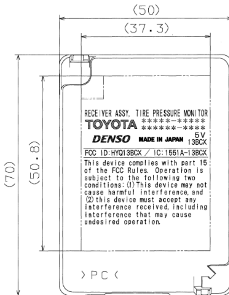
Fig7.1. Marking location and layout of receiver
