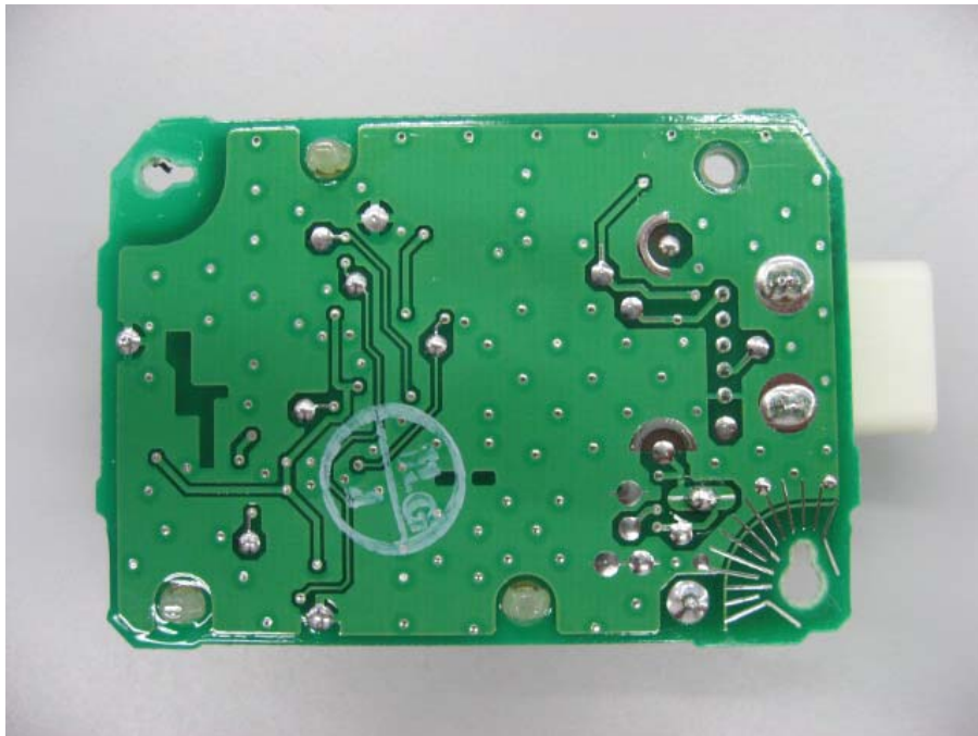
Solder Side
