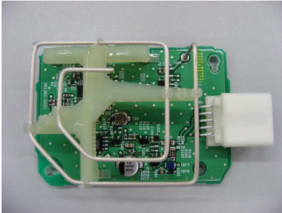
Component Side
