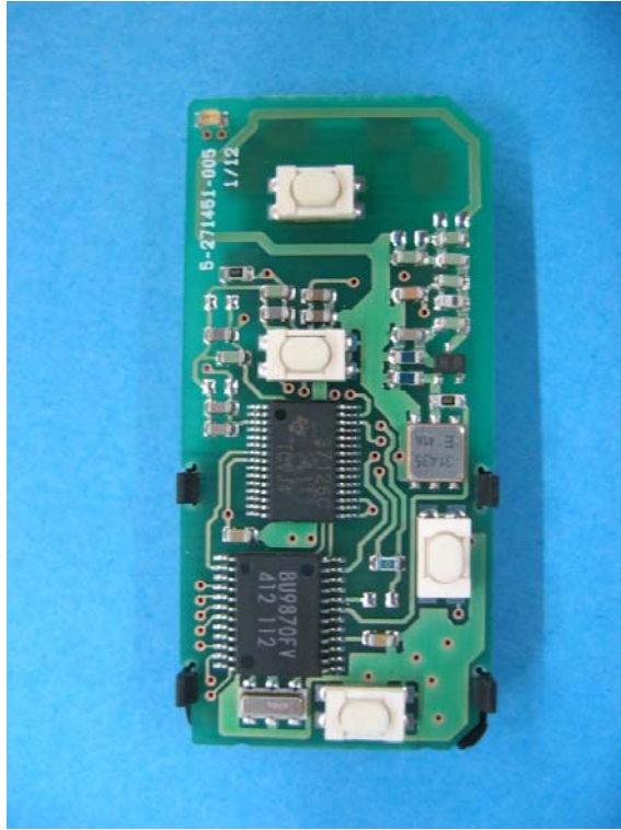
Comp side
