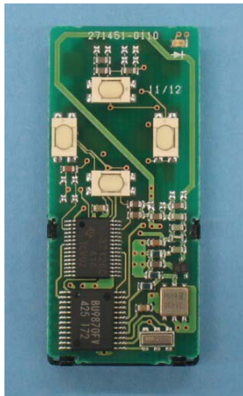
Comp Side
