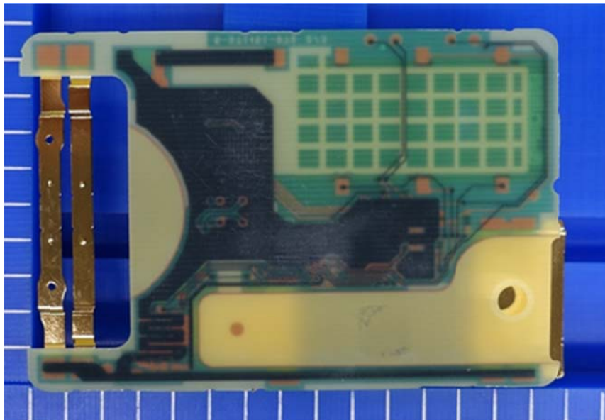
Solder Side
