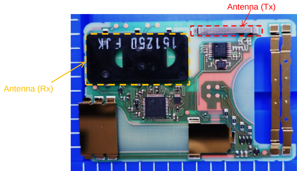
Component side
