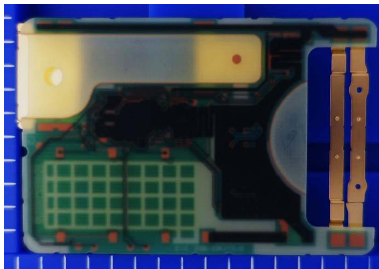
Solder side
