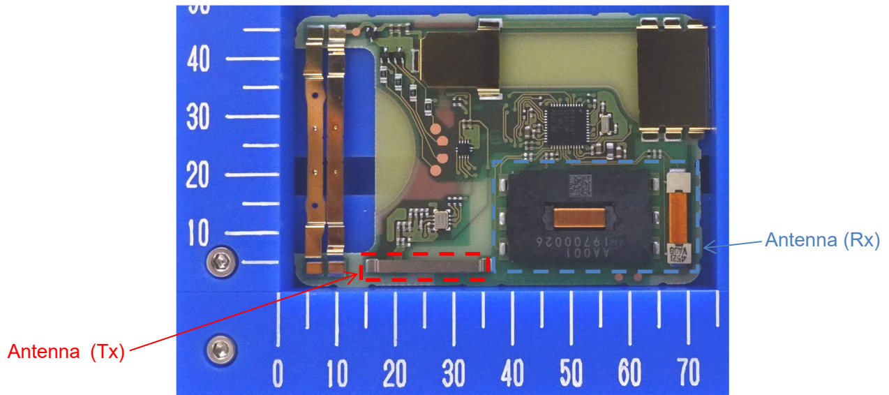
Component side
