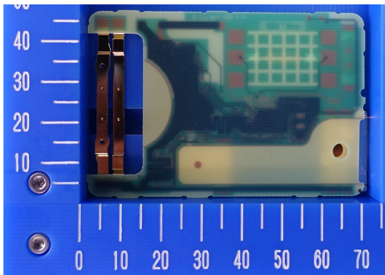
Solder side
