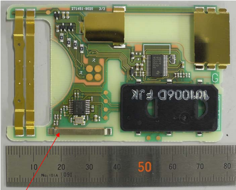
Component Side
