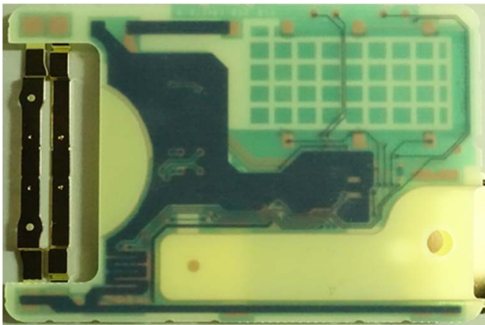
Solder side
