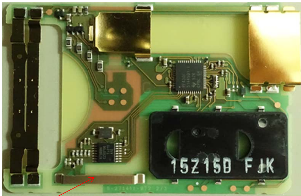
Component side
