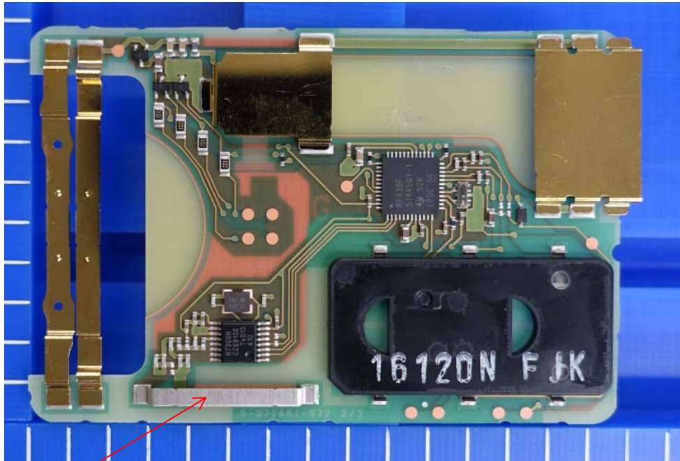
Component side
