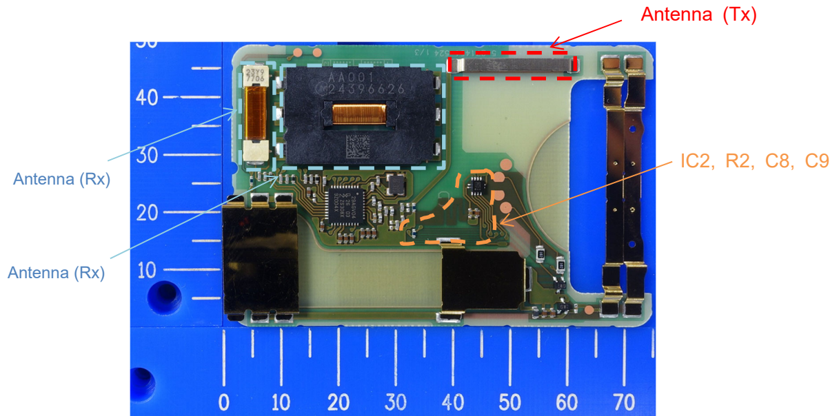
Component side
