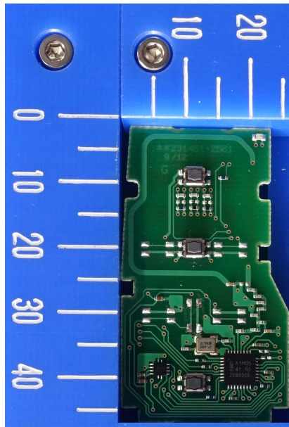
3-Button type
