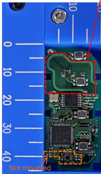
4-Button type
