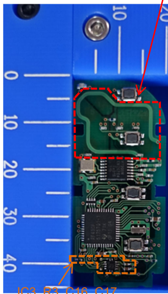
4-Button type
