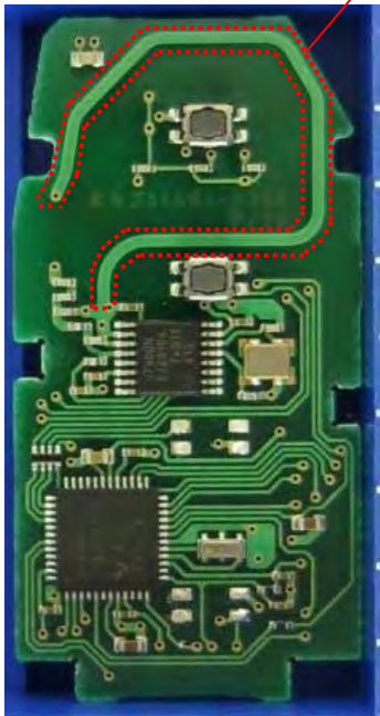
2-Button
